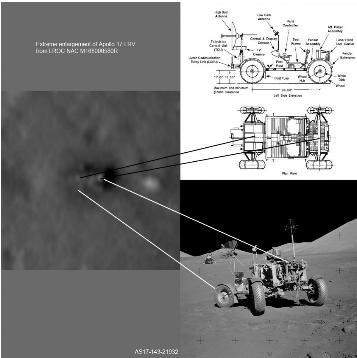
Figure 18: Extreme Enlargement of Apollo 17 LRV – 2011. The graphic shows an enlargement of the LRV (left), an image of the LRV in its final parking spot (bottom right), and a schematic of the LRV (upper right). The enlarged image was taken by the Lunar Reconnaissance Orbiter (LRO). Image Credit: NASA/GSFC/Arizona State University, M168000580R. This and other LRO digital images are archived by NASA/GSFC/Arizona State University at: http://www.lroc.asu.edu/featured_sites/#ApolloLandingSites
