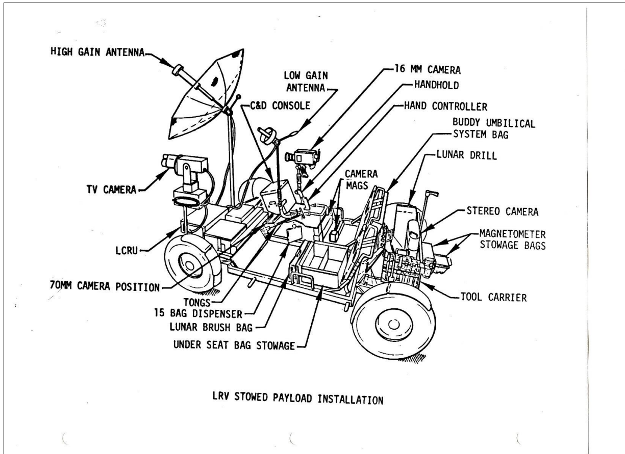
Figure 28: NASA-Marshall Space Flight Center. News release of LRV Line Drawing: LRV Stowed Payload Installation. Photo 0-10844. Release date March 1, 1971. The Boeing Company, Corporate Archives. Bellevue, WA.
