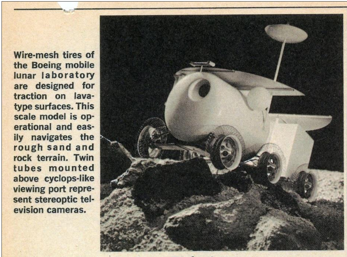
Figure 33: Illustration of Boeing's MOLAB, a precursor to the lunar roving vehicle. It featured six wheels, a pressurized cabin, and it weighed nearly 8,000 pounds. Boeing News , Jun. 3, 1965, p. 4.
