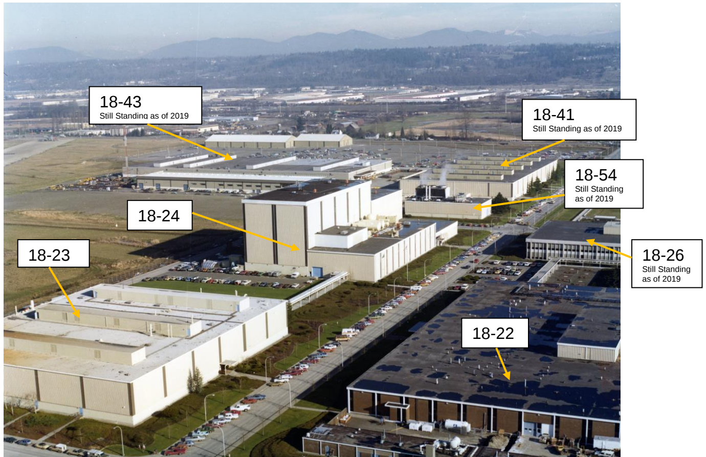
Figure 37: Boeing Space Center, 1970s. Building 18-23, where LRV fabrication, manufacturing, and assembly occurred, is located in the left foreground. Building 18-24, where the LRV was tested, is located in the middle of the photo. Courtesy: The Boeing Company, Corporate Archives. Bellevue, WA.
